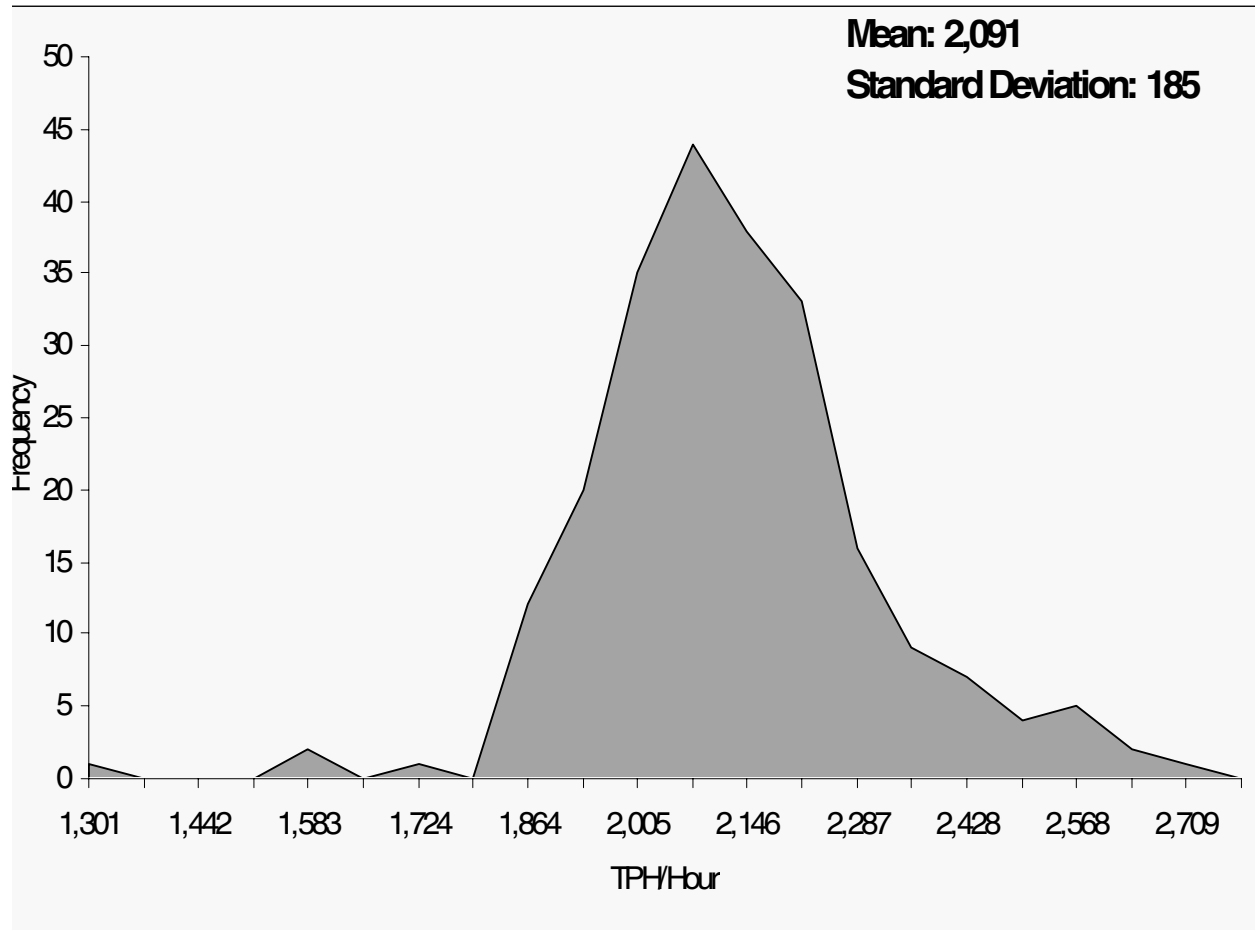
Figure C-7 Automated Flat Sorting Machine
